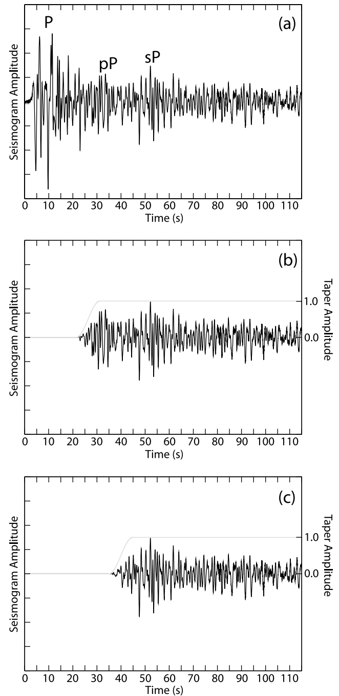
Figure 3. Effect of the taper function. (a) Seismic record from the 8 September 2008, Mw 6.9 event in Vanuatu. This record comes from station ASHH in the Hi-net array. The P , pP , and sP seismic phases are all labeled. Time is with respect to the theoretical P wave arrival. (b) The same seismic record after the taper function (light grey line) is applied at the theoretical pP arrival time. (c) Same as Figure 3b except applied to sP .
